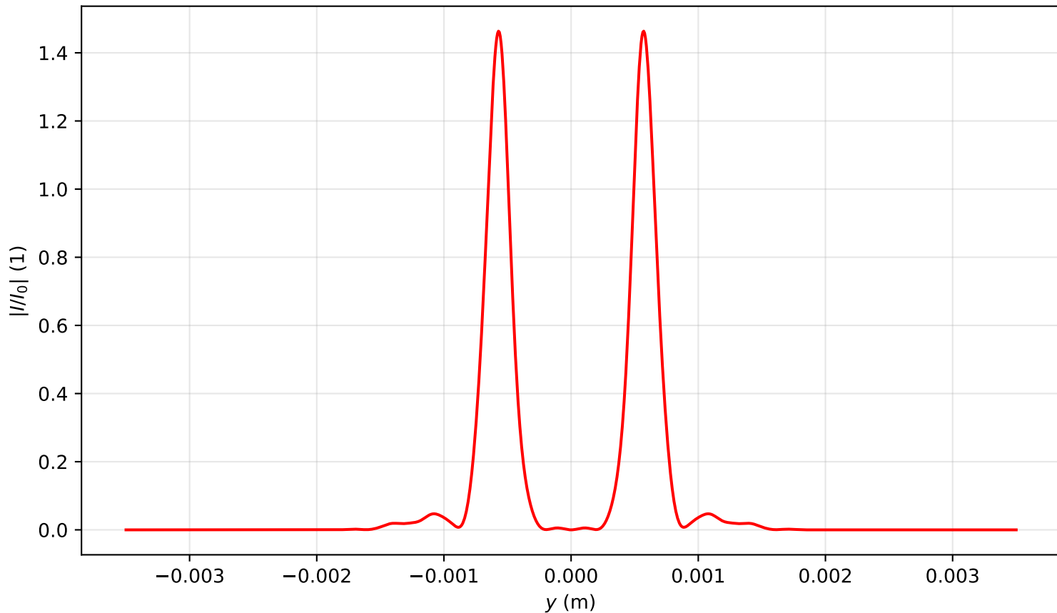
Intensity profile I(x=0, y, z=0.876)/I_0 , P_{in}=8.0P_{cr} , artificial time
